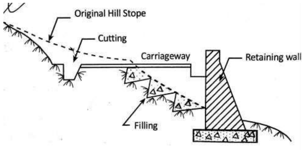
Typical Cross Sections of Hill Road
