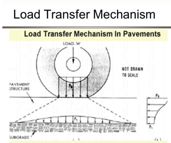
Figure 4 : Load transfer in rigid pavemet
